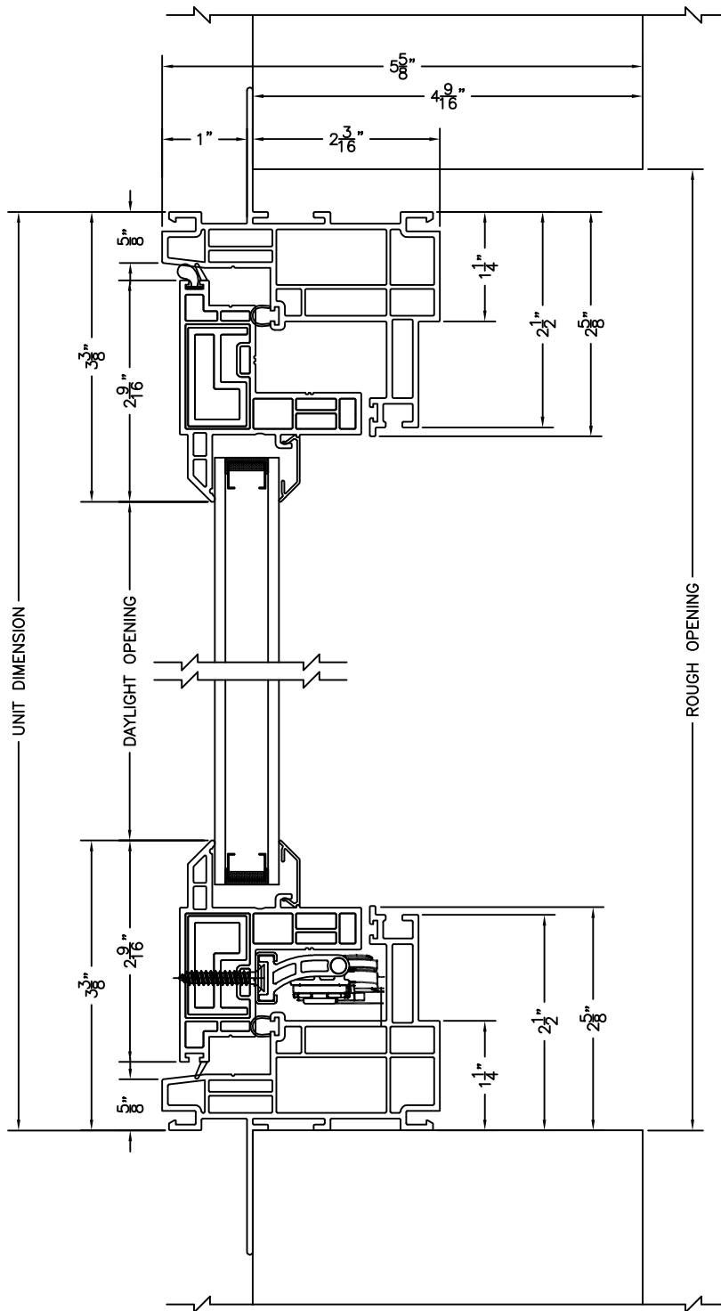
AWNING WINDOW - VERTICAL SECTION SCALE: 6" = 1' 0"
