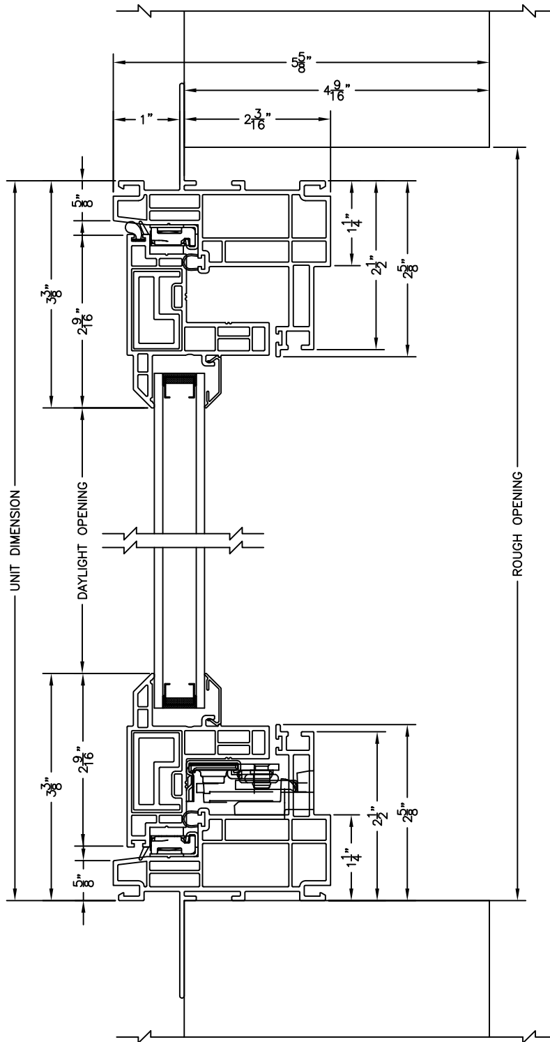
CASEMENT WINDOW - VERTICAL SECTION SCALE: 6" = 1' 0"
