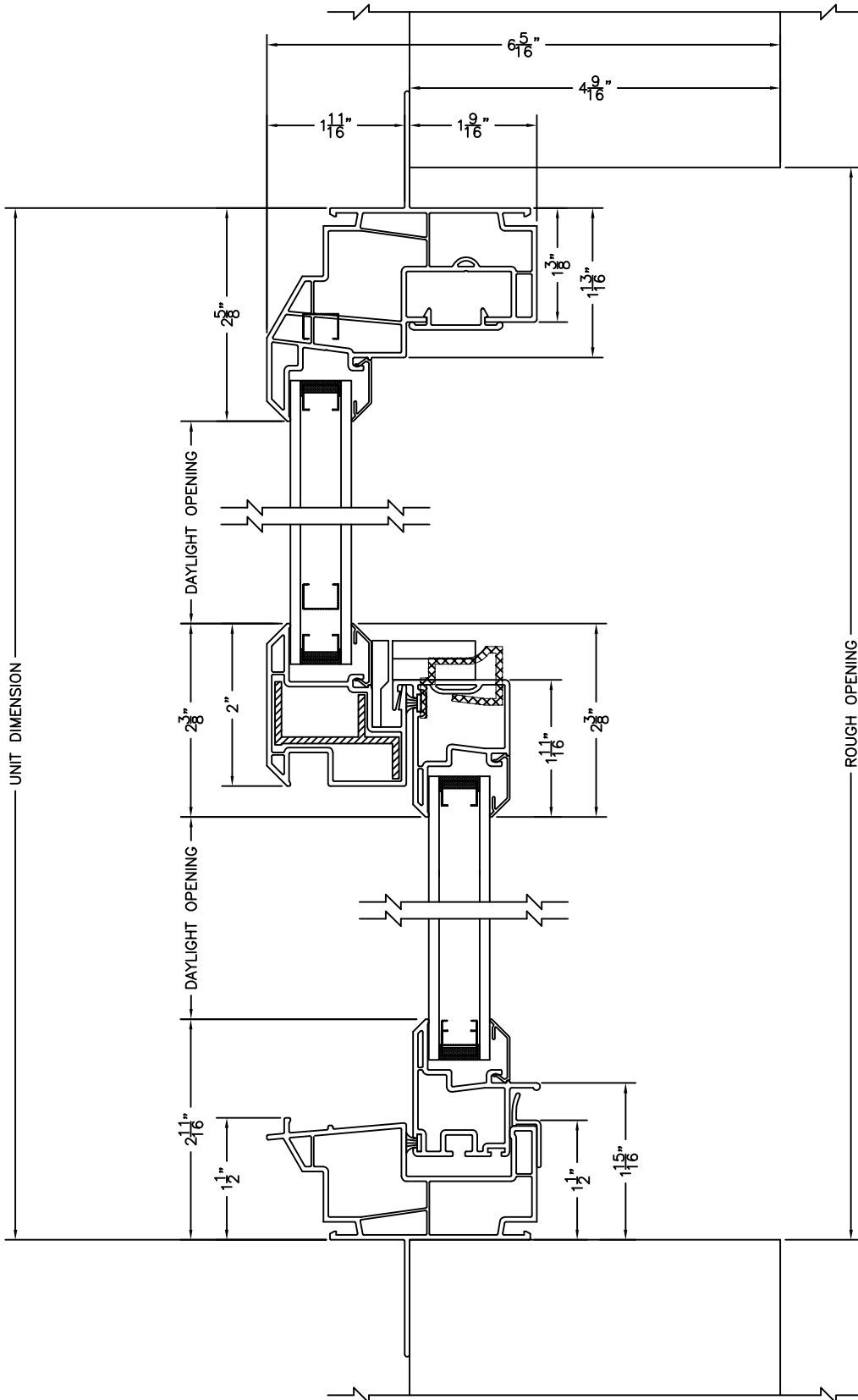
SLOPED SILL SINGLE HUNG - VERTICAL SECTION SCALE: 6" = 1' 0"
