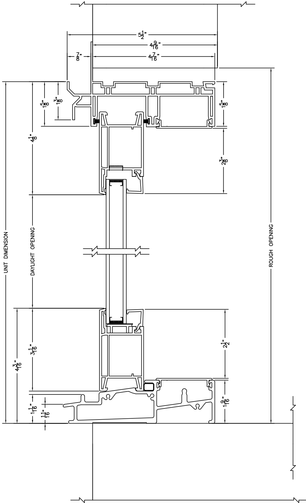
SLIDE PATIO DOOR SIDELITE - VERTICAL SECTION SCALE: 6" = 1' 0"
