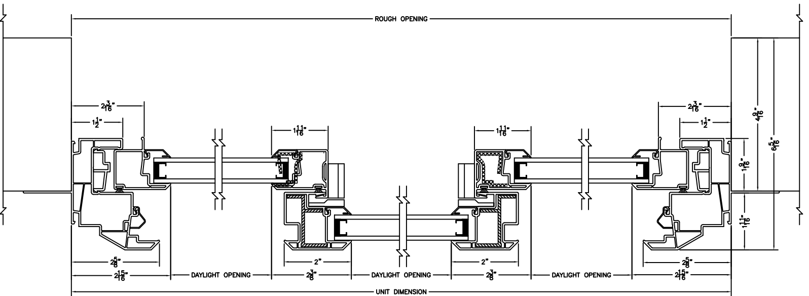
TRIPLE SLIDER - HORIZONTAL SECTION SCALE: NOT TO SCALE
