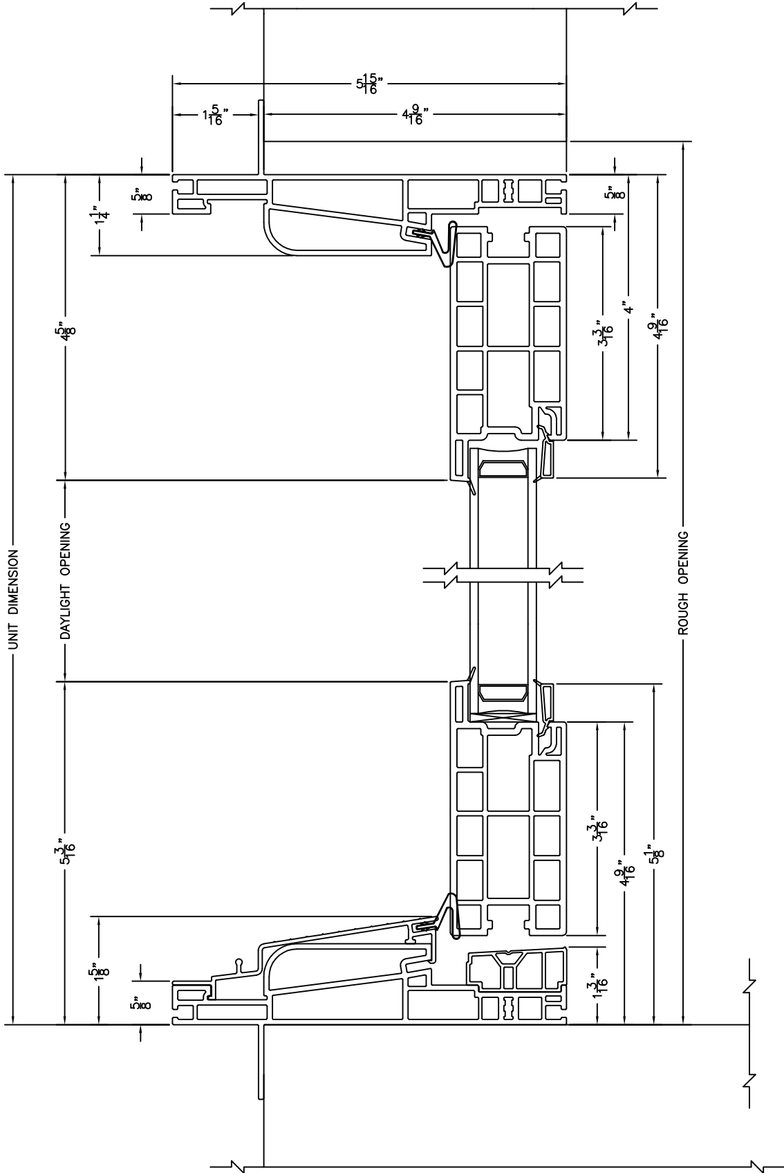
BOTANICA GARDEN DOOR - VERTICAL SECTION SCALE: 6" = 1' 0"
