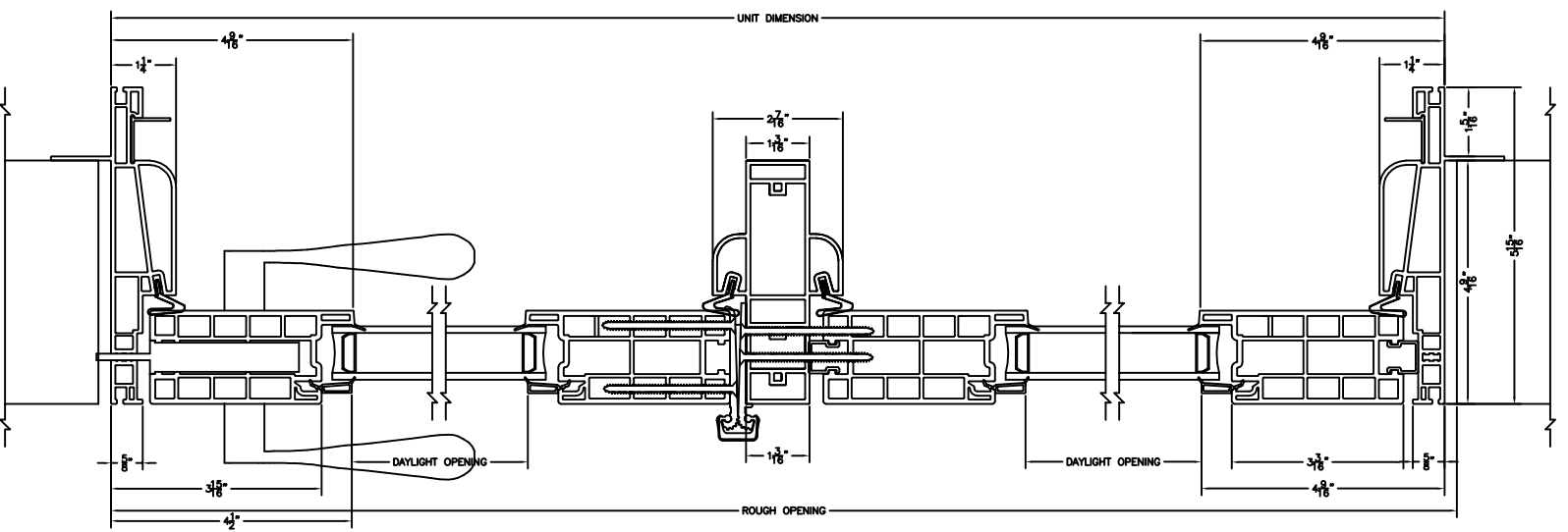
BOTANICA GARDEN DOOR FULLVIEW CENTER HINGE - HORIZONTAL SECTION SCALE: NOT TO SCALE
