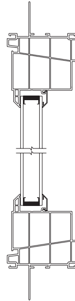
Awning Picture Window Vertical Section
