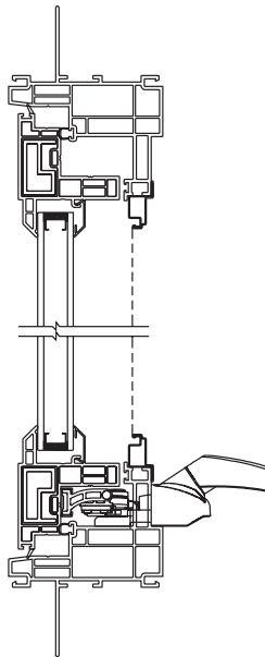
Awning Window Vertical Section
