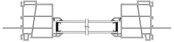
Awning Picture Window Horizontal Section
