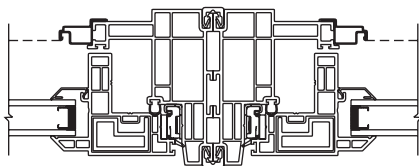
Awning Window Vertical Mull - Horizontal Section
