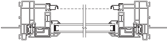
Awning Window Horizontal Section
