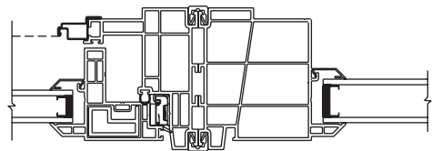
Awning Picture Window Vertical Picture Mull - Horizontal Section
