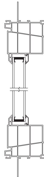
Casement Picture Window Vertical Section
