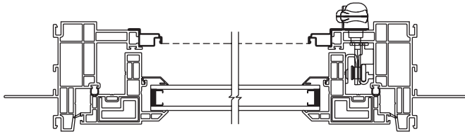
Casement Window Horizontal Section
