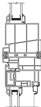
Casement Window w/Transom Mull – Vertical Section
