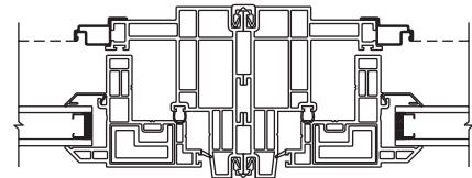
Casement Window Vertical Mull – Horizontal Section
