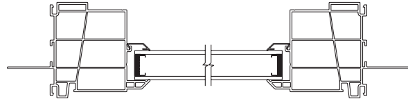
Casement Picture Window Horizontal Section
