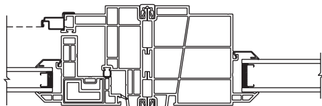
Casement Picture Window Vertical Picture Mull – Horizontal Section
