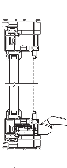
Casement Window Vertical Section
