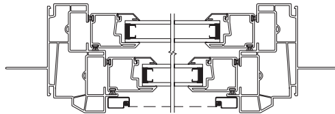
Double Hung Horizontal Section
