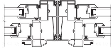
Double Hung Vertical Mull – Horizontal Section
