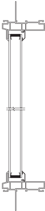
Double Hung Picture Studio – Vertical Section
