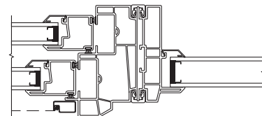
Double Hung Picture Mull – Horizontal Section
