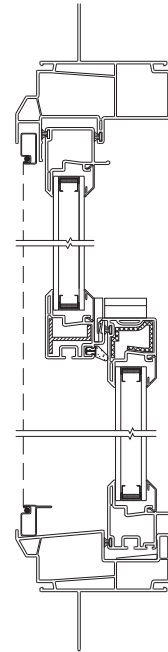
Double Hung Vertical Section
