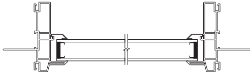
Double Hung Picture Studio – Horizontal Section
