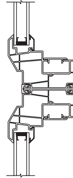
Single Hung Window Picture Mull – Vertical Section
