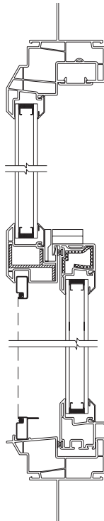
Single Hung Sloped Sill – Vertical Section
