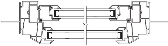
Single Hung Mainframe – Horizontal Section
