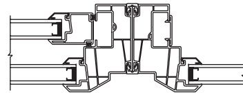
Single Hung Picture Mull – Horizontal Section
