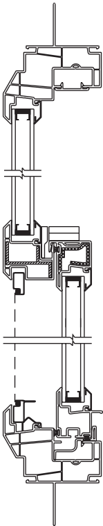
Single Hung Main Frame – Vertical Section
