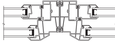
Single Hung Window Horizontal Section
