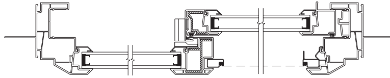
Single Slide Window Horizontal Section
