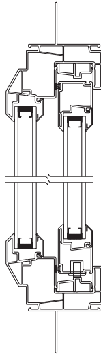
Single Slide Window Vertical Section
