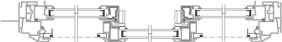
Triple Slide Window Horizontal Section
