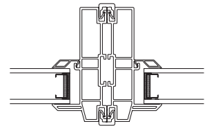
Direct Set Frame Mull – Horizontal Section
