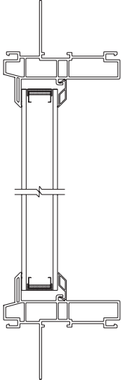
Direct Set Vertical Section
