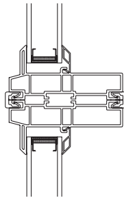
Direct Set Frame Mull – Vertical Section
