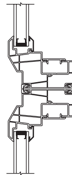
Specialty Transom Horizontal Mull – Vertical Section
