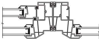
Specialty Vertical Picture Mull – Horizontal Section
