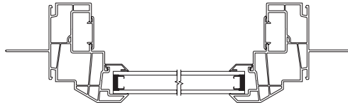
Specialty Horizontal Section
