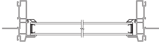
Direct Set Horizontal Section
